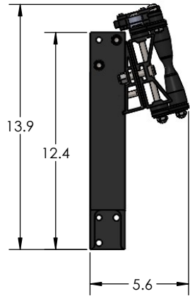
STORAGE POSITION
