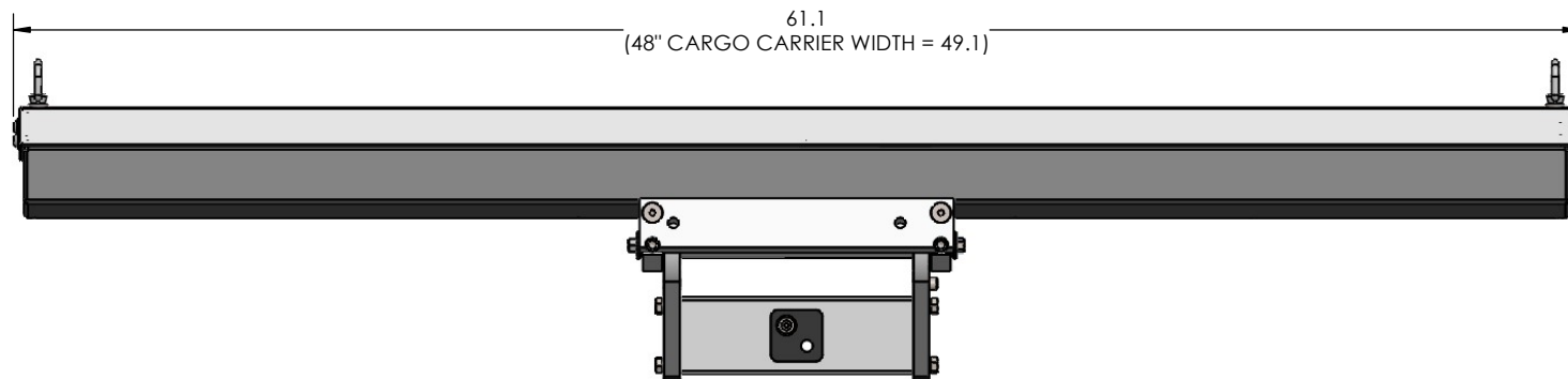
OVERALL WIDTH
