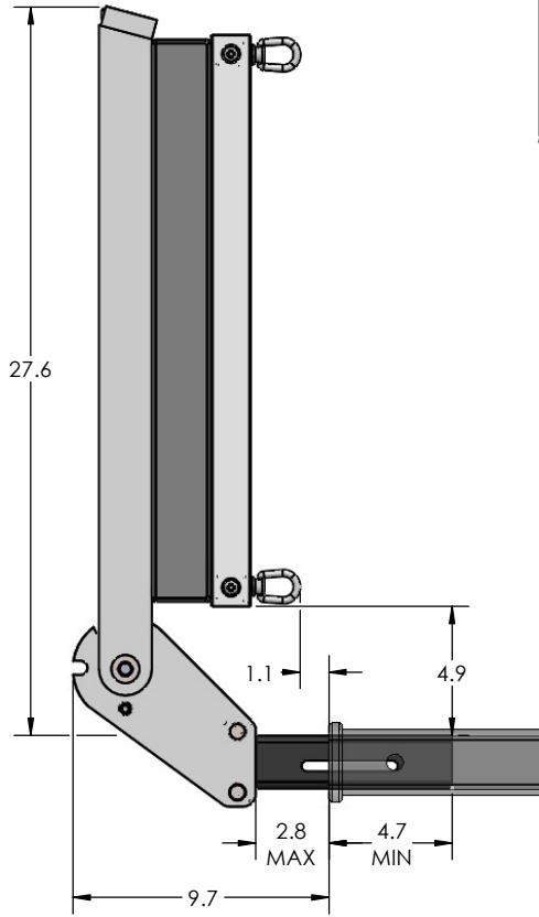
STORAGE POSITION
