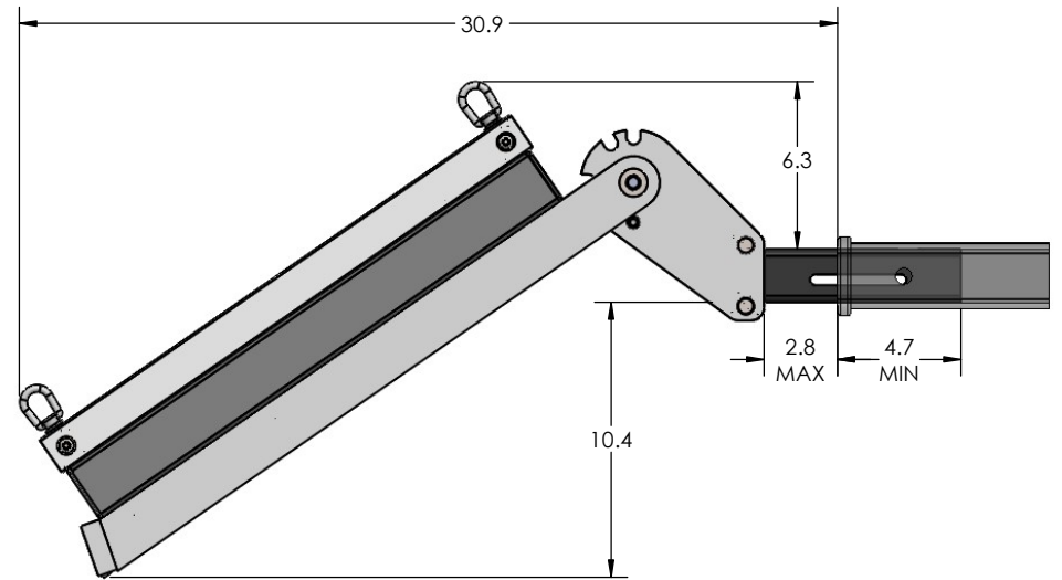
DOWN POSITION
