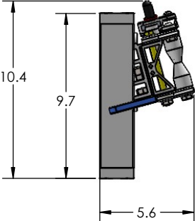
STORAGE POSITION
