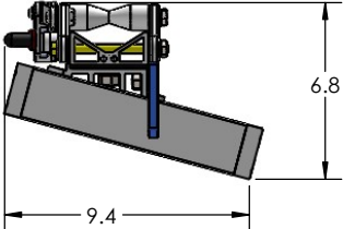
RIDE POSITION
